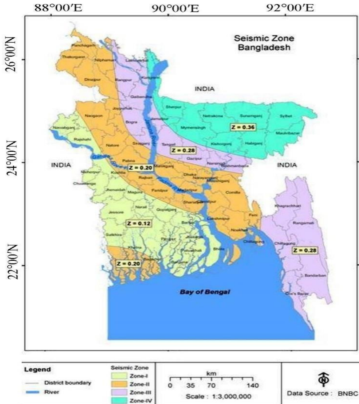
Figure 3: Seismic Zone Map of Bangladesh BNBC -2020
